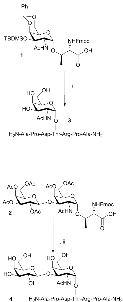
Scheme 1 Solid-phase synthesis of glycopeptides 3 and 4 . Reagents and conditions: (i) glycopeptide synthesis according to the Fmoc protocol. (ii) Deacetylation with NaOMe/MeOH, 20 mM.
