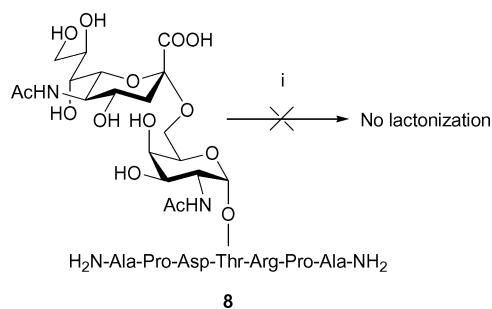
Scheme 4 Lactonization of sialylated glycopeptide 8 . Reagents and conditions: (i) glacial acetic acid (AcOH- d 4 ), RT.
