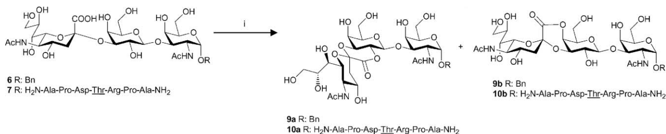
Scheme 3 Lactonization of sialylated benzyl glycoside 6 and sialylated glycopeptide 7 . Reagents and conditions: (i) glacial acetic acid (AcOH- d 4 ), RT.
