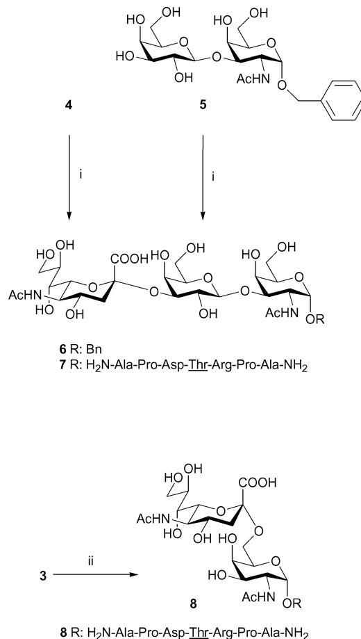
Scheme 2 Enzymatic sialylation of benzyl glycoside 5 and glycopeptides 3 and 4 . Reagents and conditions: (i) CMP-Neu5Ac (1.75 equiv), \alpha 2,3OST, 0.25 M sodium cacodylate buffer (pH 6) containing 0.1% Triton X-100, 37 °C. (ii) CMP-Neu5Ac (2 mM), ST6GalNAc-I, 20 mM Bis-Tris buffer (pH 6.5) containing EDTA (20 mM) and dithiothreitol (1 mM), 37 °C.
